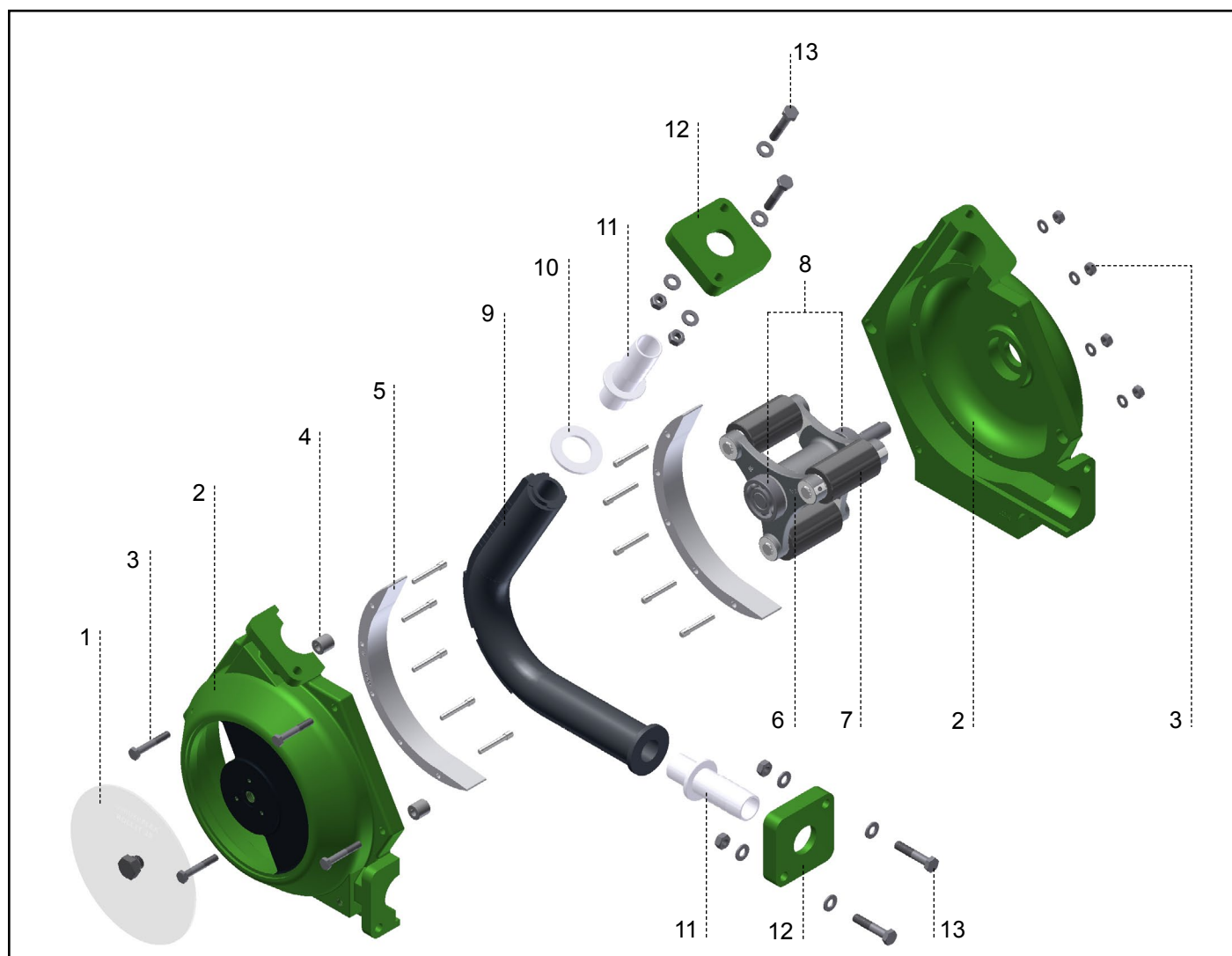
Figure 2 Layout - Rollit 15-50 exploded view
